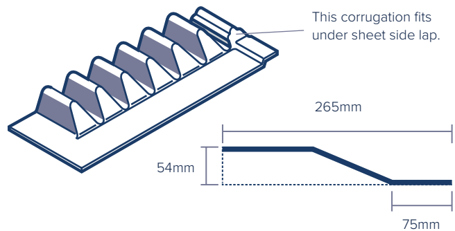
Fig.2 Eaves Closure
