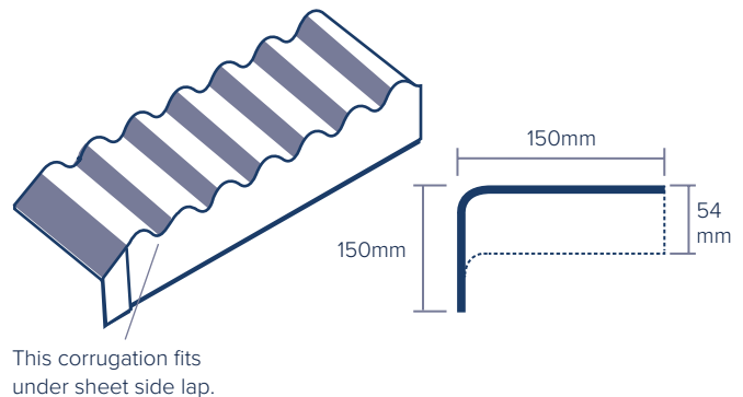
Fig.2 Eaves Closure
